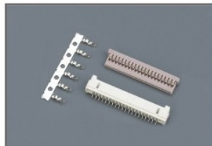
DF14(1.25mm) P14
