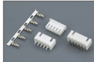
TJC3(2.50mm) P39
