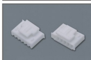
HA(2.50mm) P50
